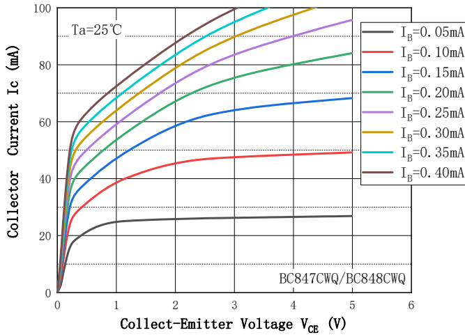
Fig. 3-Static Characteristic
