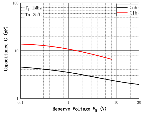
Fig. 8 - Cob/Cib— V_{CB}/V_{EB}
