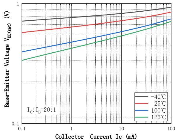
Fig. 6 - Base-Emittor Voltage
